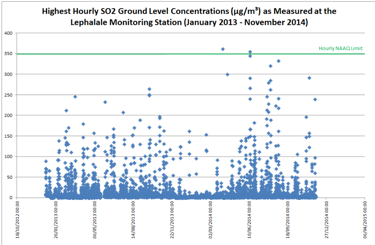
Figure 3-8: Hourly SO 2 measured at the Lephalale monitoring station for the period January 2013 to November 2014
