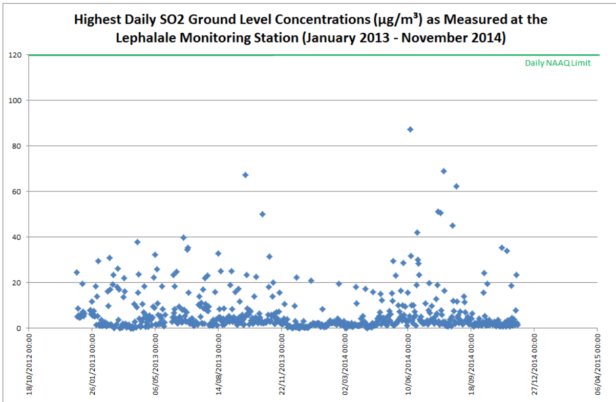
Figure 3-9: Daily SO 2 measured at the Lephalale monitoring station for the period January 2013 to November 2014
